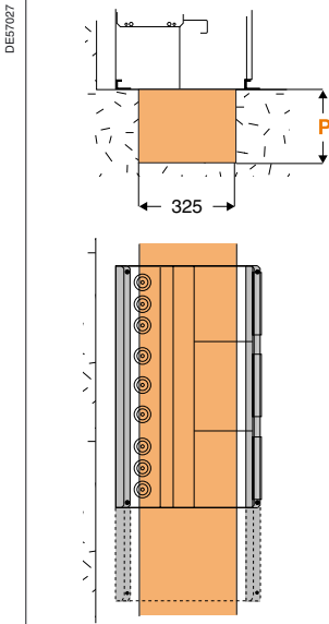
Cable entry through a trench
