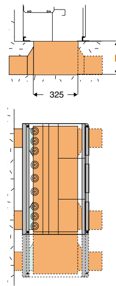
Cable entry through a duct
