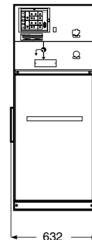
RM6 1 functional unit circuit breaker
