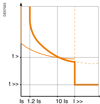
With IDMT low set point
