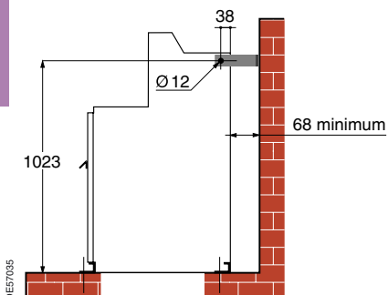
RM6 3 or 4 functional units with extensibility module
